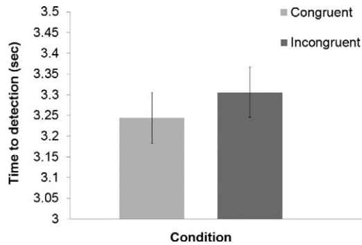
Figure 2. Mean detection time by congruency. Note significantly reduced suppression time when hand posture and task-irrelevant visual hand are congruent. Error bars are SEM .
