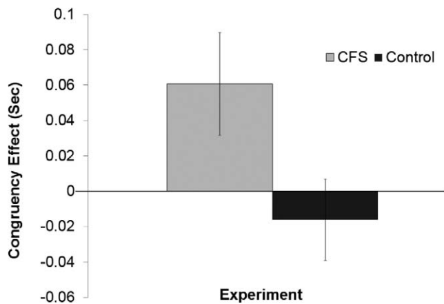
Figure 3. Congruency effect in the CFS and non-CFS experiments. The congruency effect (incongruent-congruent) in the CFS experiment was positive and significant. No such effect was found in the non-CFS control experiment. Error bars are SEM.
