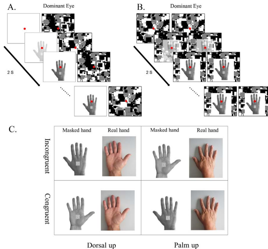
Figure 1. Experimental design. (A) CFS experiment, Mondrian masks were presented to the dominant eye. The target image presented to other eye was either congruent or incongruent with the participant's hand position. (B) Control experiment. Similar stimuli were presented to both eyes; hence, no binocular suppression. (C) A 2 \times 2 full factorial design. Gray-scale hands are the task-irrelevant visual stimuli presented to the nondominant eye. Color hands represent the nonvisible hand position of the participant. Participants were required to indicate the orientation of lines in the square of the visually presented hand stimuli.
